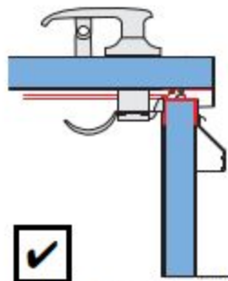
L04 External Handle Padlock External
