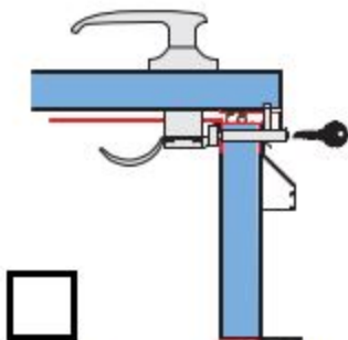
L06 Euro Deadlock Thumb Turn Inside external key lock (Not Pictured)
