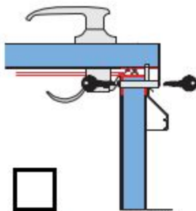
L07 Euro Deadlock Internal and external key lock (Not Pictured)
